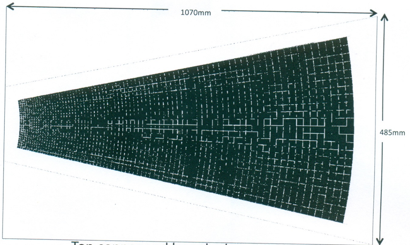
Top copper and board edge
